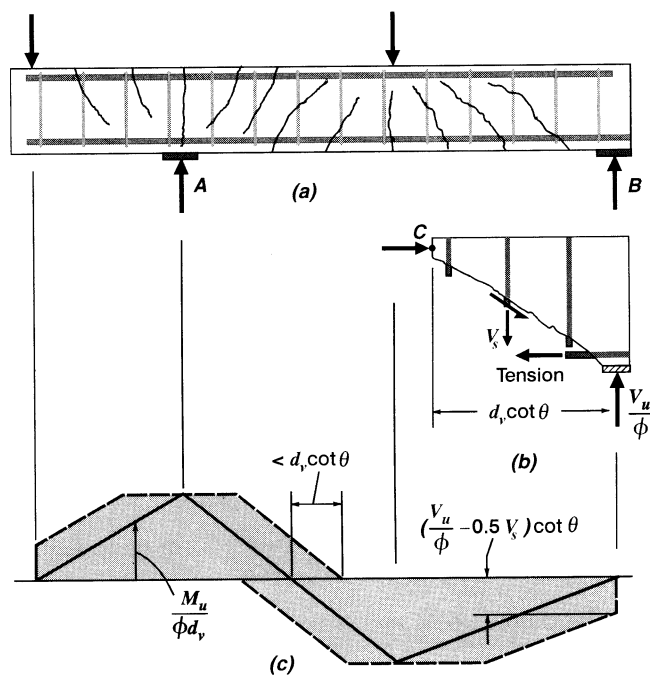
Fig. 8—Influence of shear on forces in longitudinal reinforcement
